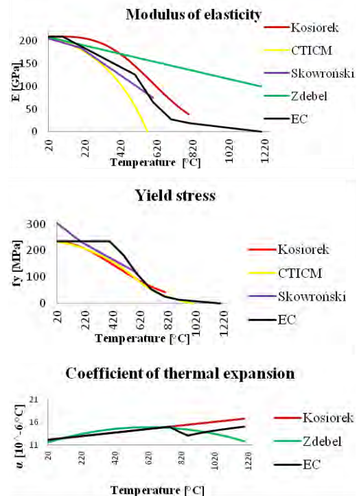
Fig. 1. The mechanical properties of steel at elevated temperature
