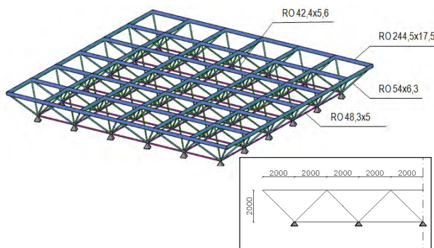
Fig. 3. The geometry of the analyzed structural roof
