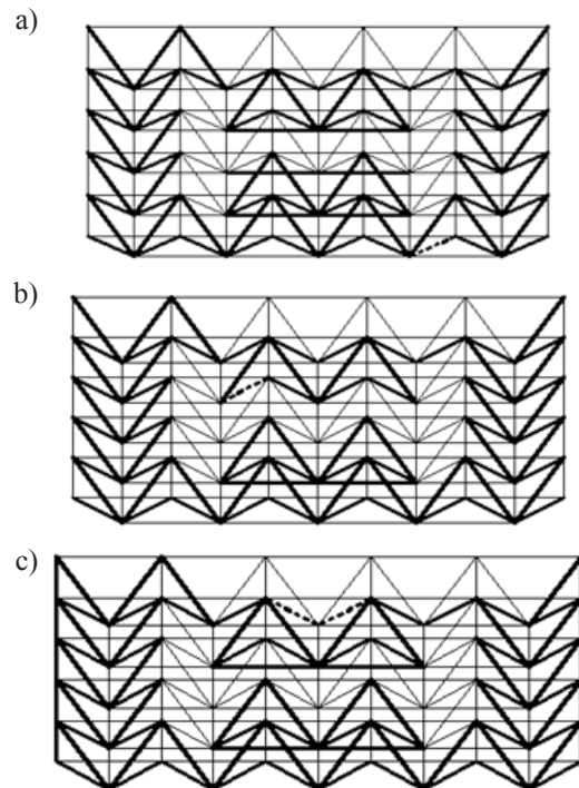
Fig. 5. The results of fire analysis with reference to: a) temperature, b) bearing capacity, c) time
